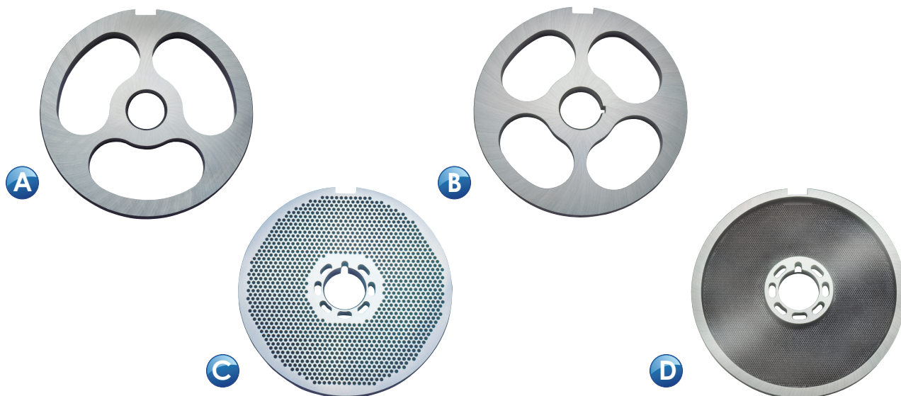
B 8 5/8" Kidney-hole plates #2084, Keyway center, 8 5/8" O.D. 2 1/8" I.D.
