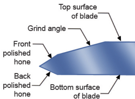
Typical skinner blade profile
