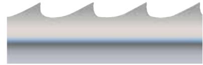
Style #322 - 3 teeth/in. Gauge .022 Width 5/8"
