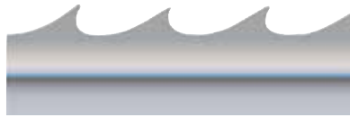
Style #332P - 3 teeth/in. Gauge .032 Width 1"
