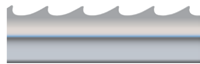
Style #422 - 4 teeth/in. Gauge .022 Width 5/8"
