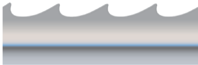
Style #325P - 3 teeth/in. Gauge .025 Width 3/4"
